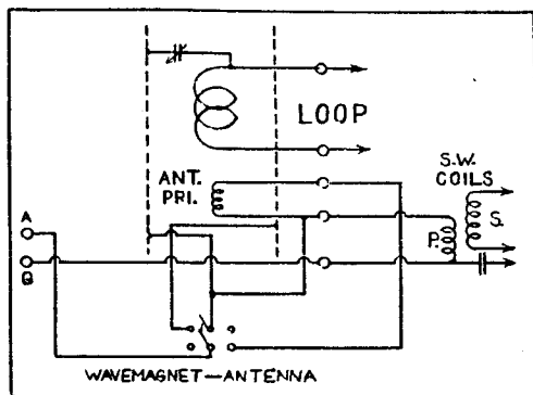
WAVEMAGNET CIRCUIT
