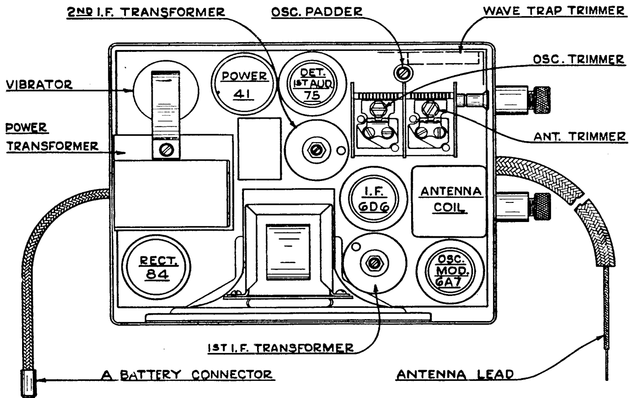
Fig. 2.—Tube Position. 5-M-90
