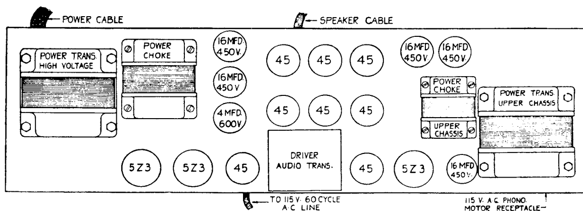
Power Pack Chassis Drawing
