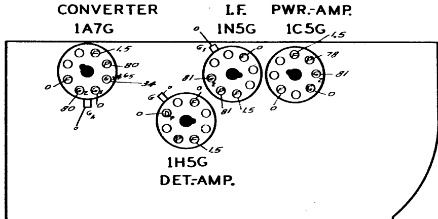
FRONT OF CHASSIS
