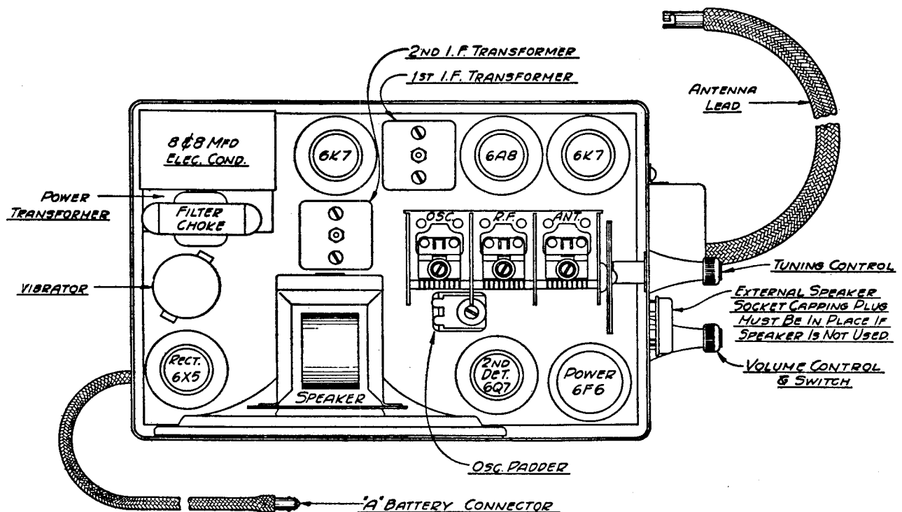
Fig. 5.—Tube Position. 6-M-92
