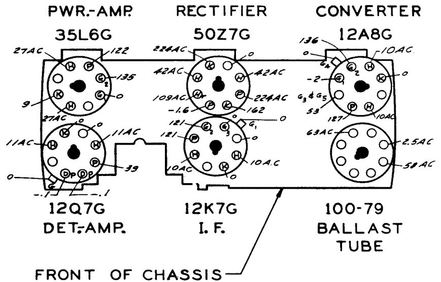
Socket Voltages
