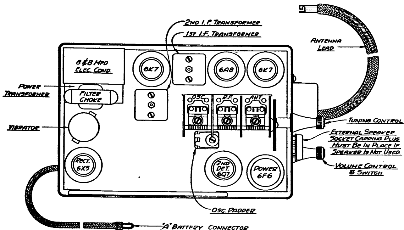
Fig. 11.—Tube Position. 6-M-91S, 6-M-91D
