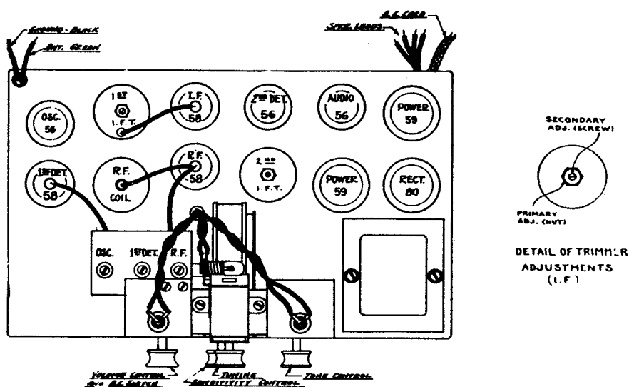
TUBE POSITION
