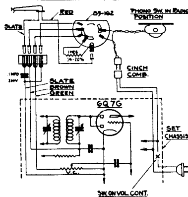
CIRCUIT #3A MODEL #6D-302-CHASSIS #5646 WIRING OF PHONO CKT. COMPONENTS
