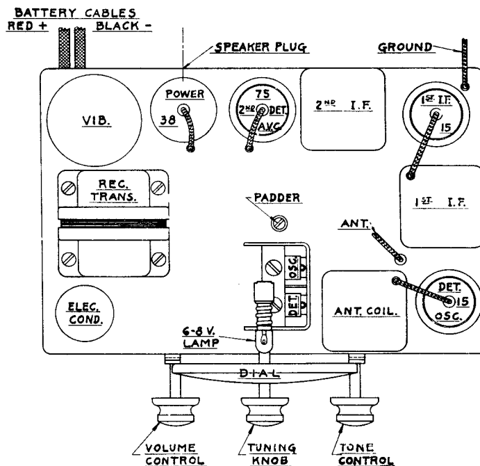
Tube Layout
