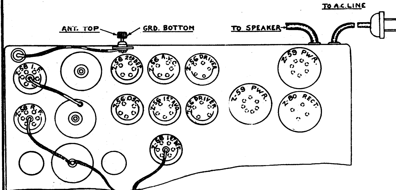
TUBE LAYOUT
