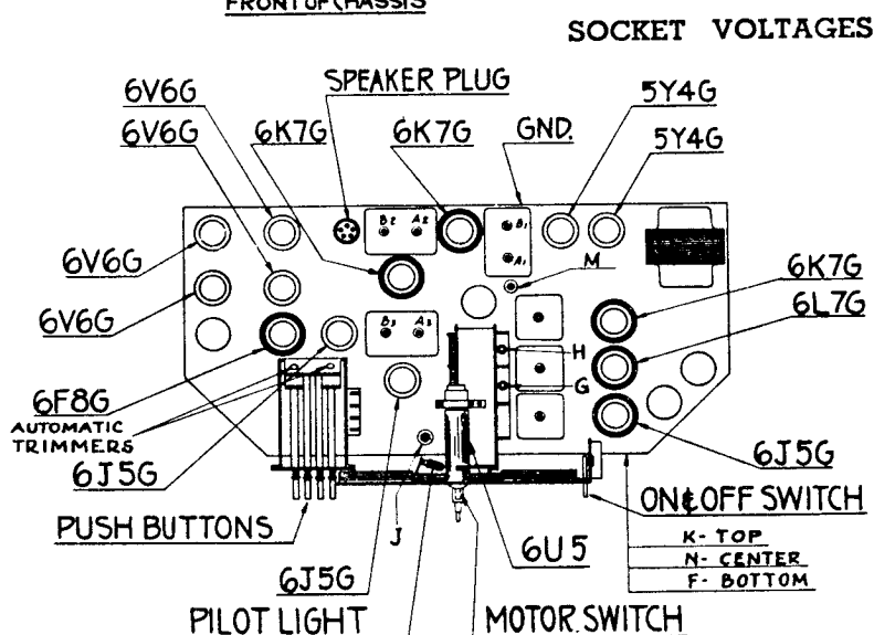
Location of Tubes and Trimmers
