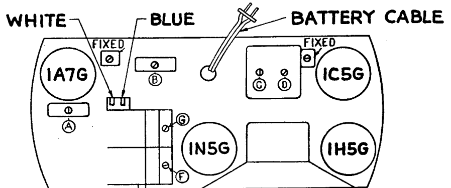
Location of tubes and trimmers
