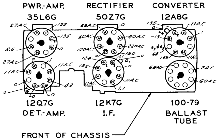
Socket Voltages
