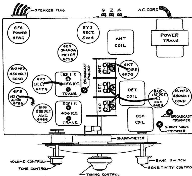
TUBE POSITION
