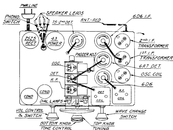
Tube Position
