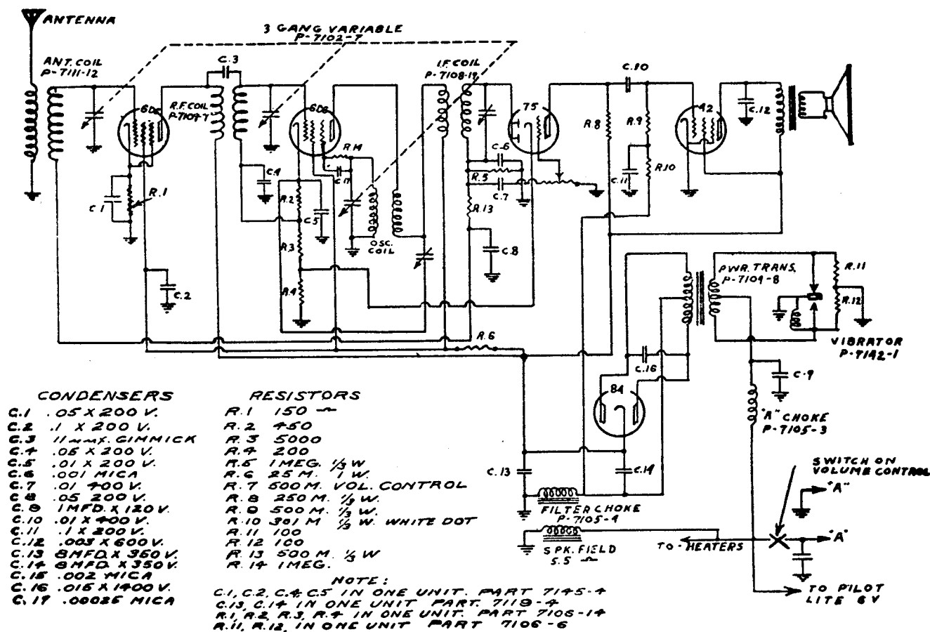
CIRCUIT DIAGRAM - MODEL 7
