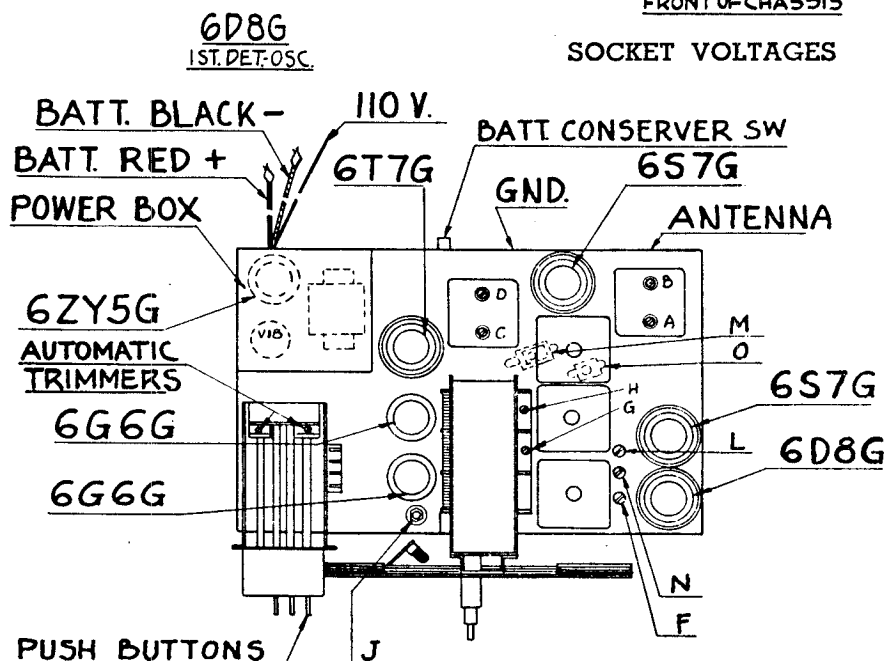
Location of Tubes and Trimmers
