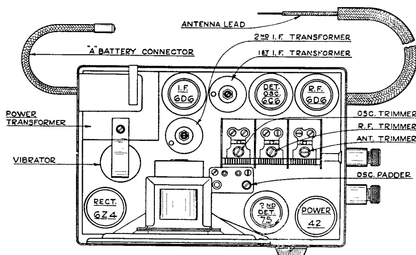
Fig. 1—TUBE POSITION
