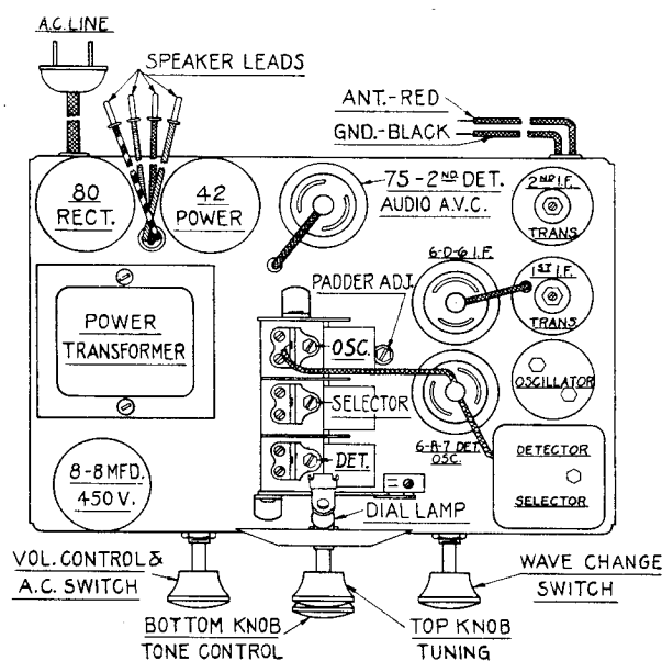
Tube Position
