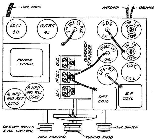
TUBE-POSITION Tube Position
