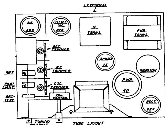
TUBE POSITION
