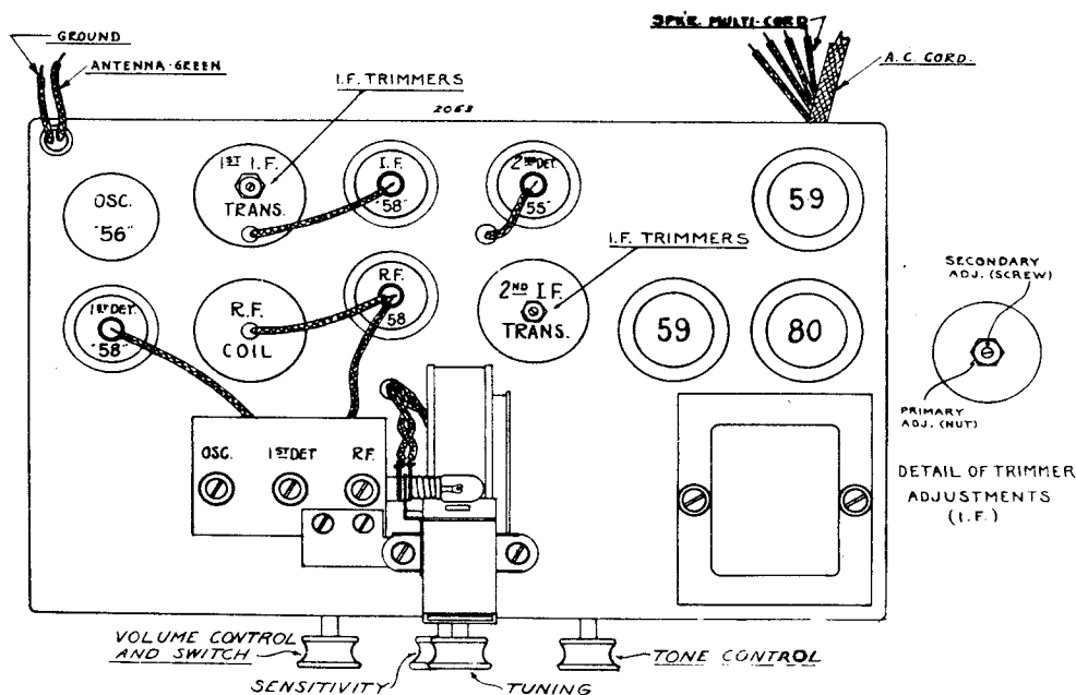
TUBE POSITION
