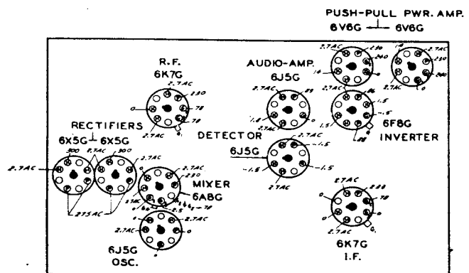
Location of Tubes and Trimmers
