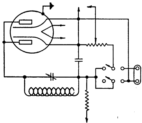
CIRCUIT CHANGES FOR PHONOGRAPH INSTALLATIONS ON CHASSIS MODELS— 5638-5710
