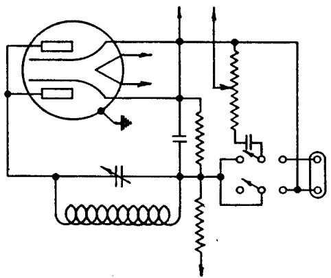
CIRCUIT CHANGES FOR PHONOGRAPH INSTALLATIONS ON CHASSIS MODELS— 5644-5644A-5702-5702A 5709AT-5905-5905A-5905AT
