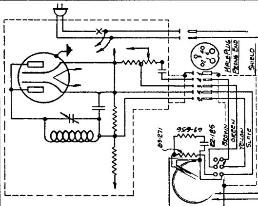
CIRCUIT CHANGES FOR PHONOGRAPH INSTALLATION ON CHASSIS MODELS— 5648-5711-5711T
