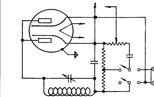
CHANGES IN CIRCUIT FOR RADIO-PHONO INSTALLATIONS ON CHASSIS MODELS— 1204-1501 1204A-1501A
