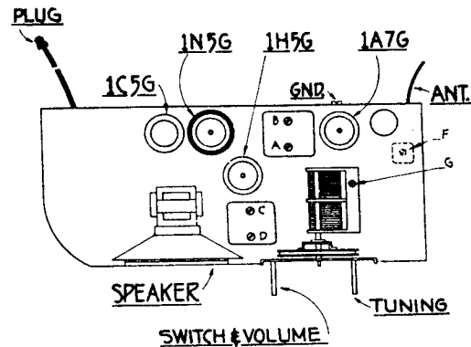
Location of tubes and trimmers
