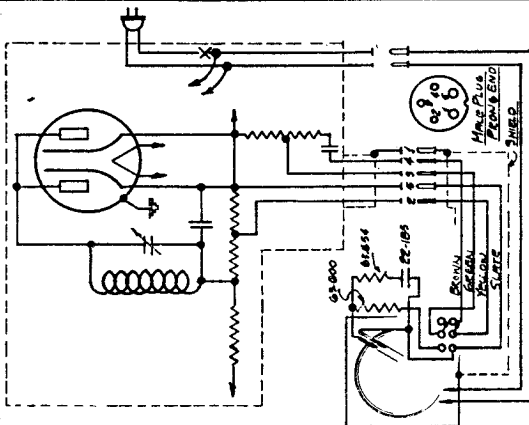
CIRCUIT CHANGES FOR PHONOGRAPH INSTALLATIONS ON CHASSIS MODELS— 5644-5644A-5702-5702A 5709AT-5905-5905A-5905AT
