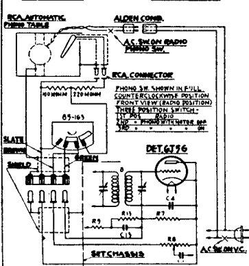
CIRCUIT #98 MODEL 95-307 CHASSIS #5907
