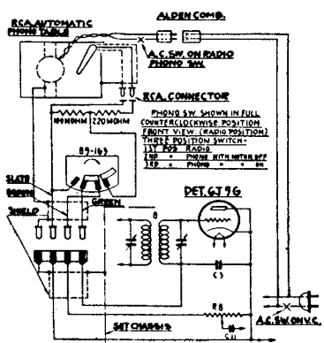
CIRCUIT # 5A MODEL-65-306 CHASSIS # 5651
