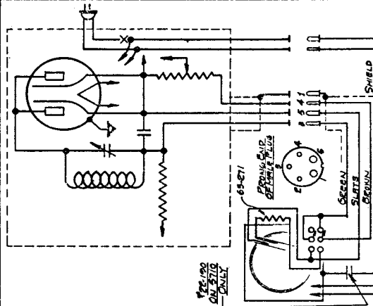
CIRCUIT CHANGES FOR PHONOGRAPH INSTALLATIONS ON CHASSIS MODELS— 5638-5710
