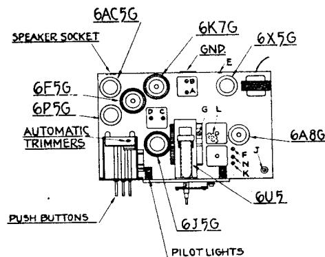
Location of tubes and trimmers
