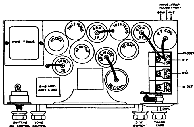
Tube Layout
