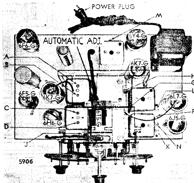
Location of Tubes and Trimmers
