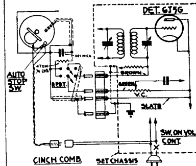
CIRCUIT #30 MODEL #65-301 & MODEL #65-305 CHASSIS #9651
