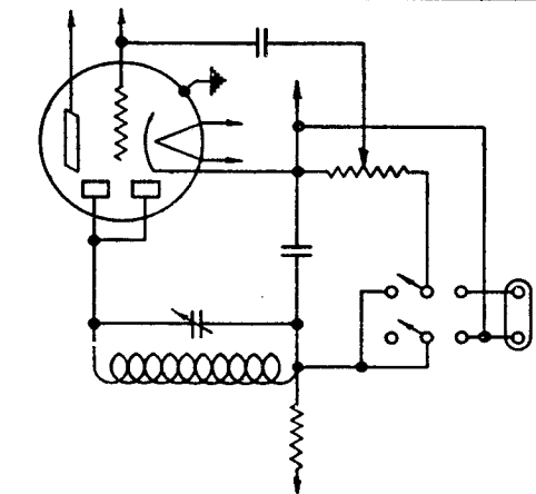
CIRCUIT CHANGES FOR PHONOGRAPH INSTALLATIONS ON CHASSIS MODELS— 5409-5521-5521A-5521AT-5523-5524 5524T-5526-5526A-5527-5529-5539
