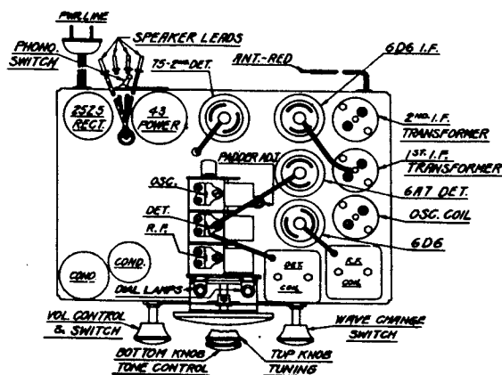
Tube Position
