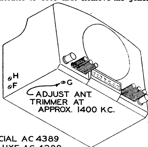
Fig. 4. Antenna Adjustment
